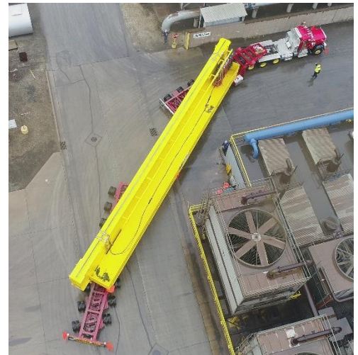
16-Axle Two Bolster Steerable Dolly - 100 Ton Capacity
